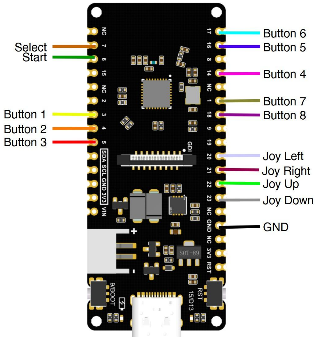
Picture 45 - ESP32-C6 DFR1075 proposed connection diagram
