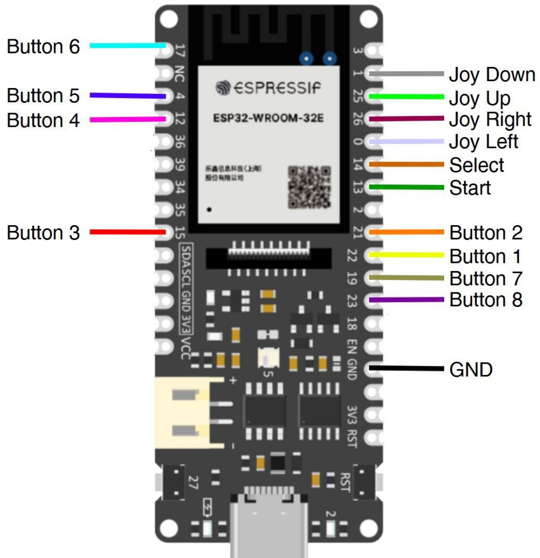
Picture 47 - ESP32-E (N16R2) DFR1139 proposed connection diagram
