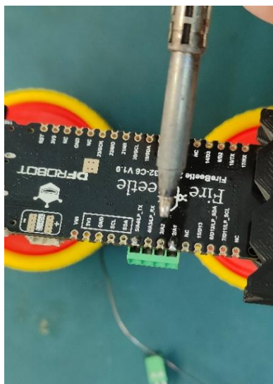
Picture 9 – soldering the terminals
