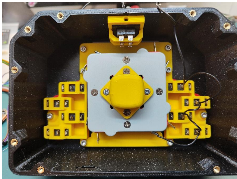
Picture 40 – daisy chaining the GND
