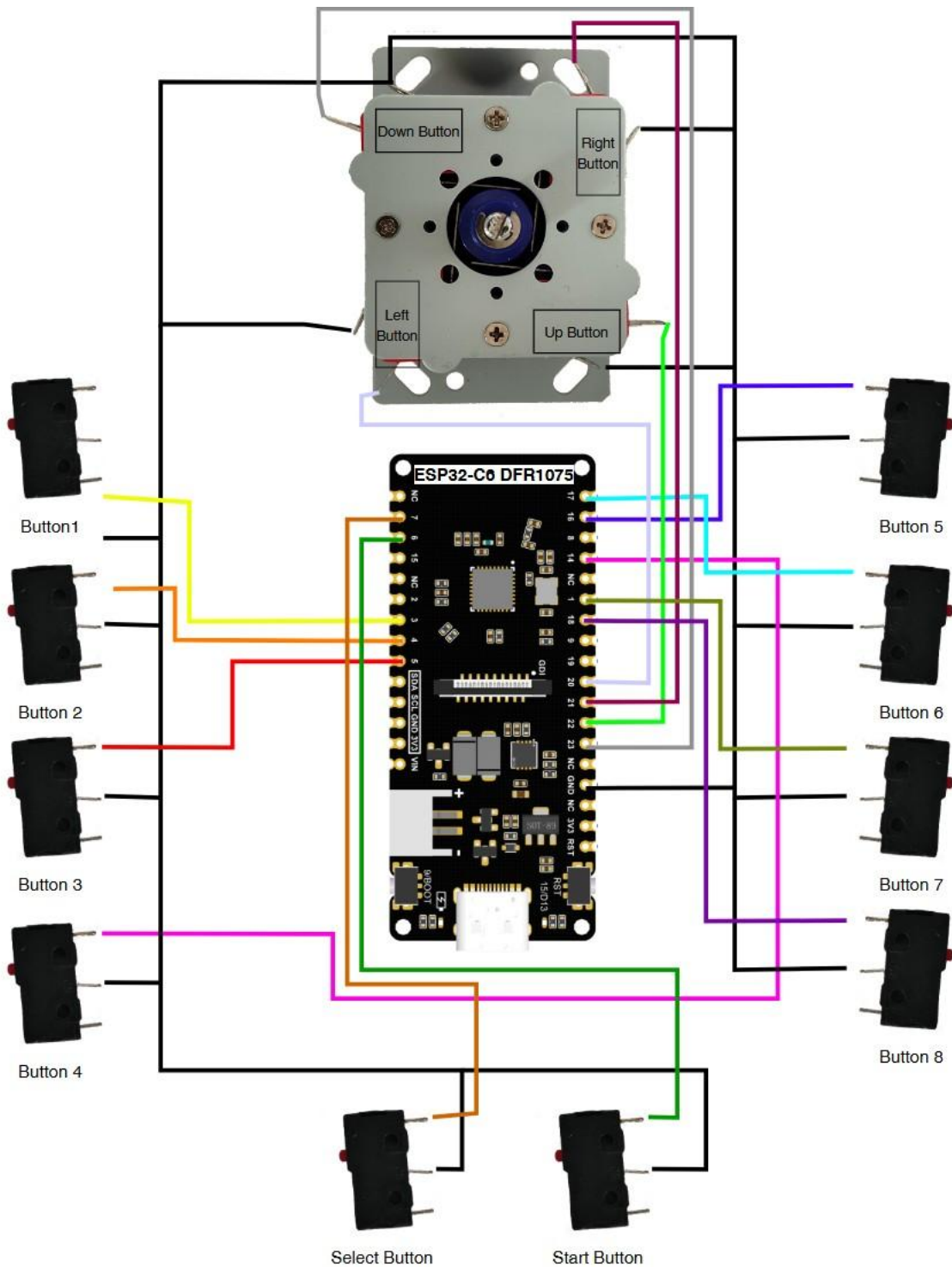
Picture 44 - Wiring Diagram for the ESP32-C6
